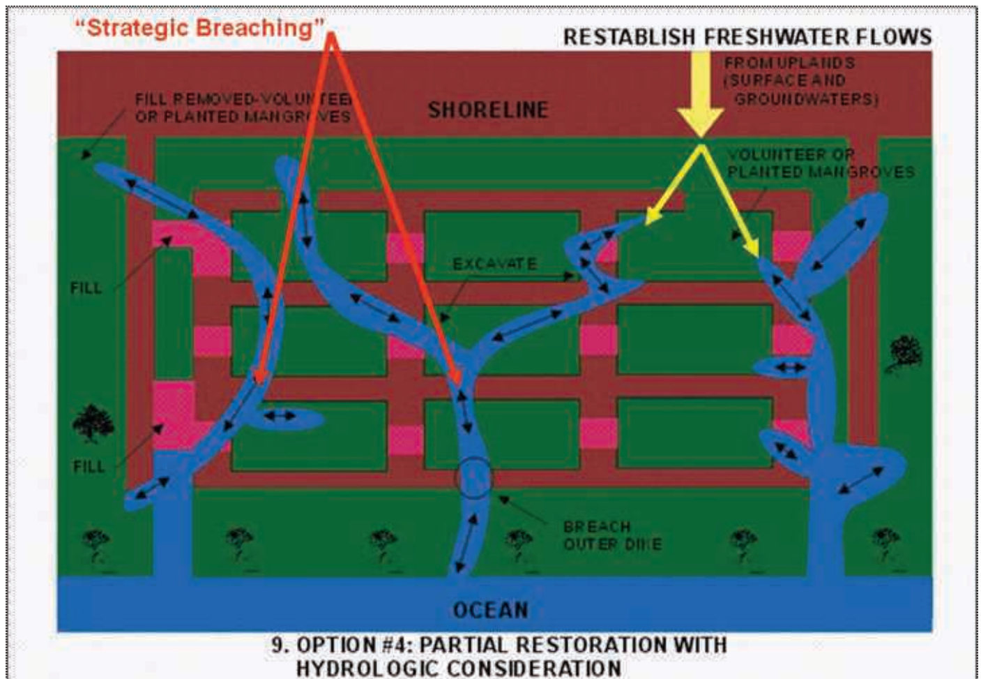
Figure x. The strategic breaching model for disused tambaks restoration back to mangroves as presented at the Regional Seminar.
