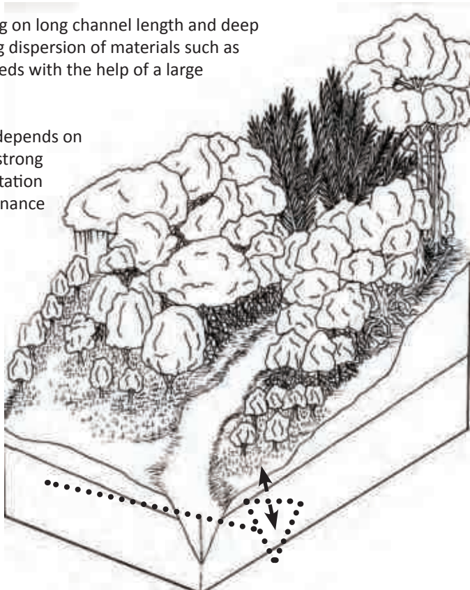
Fig 8.10 Tidal Prisms
