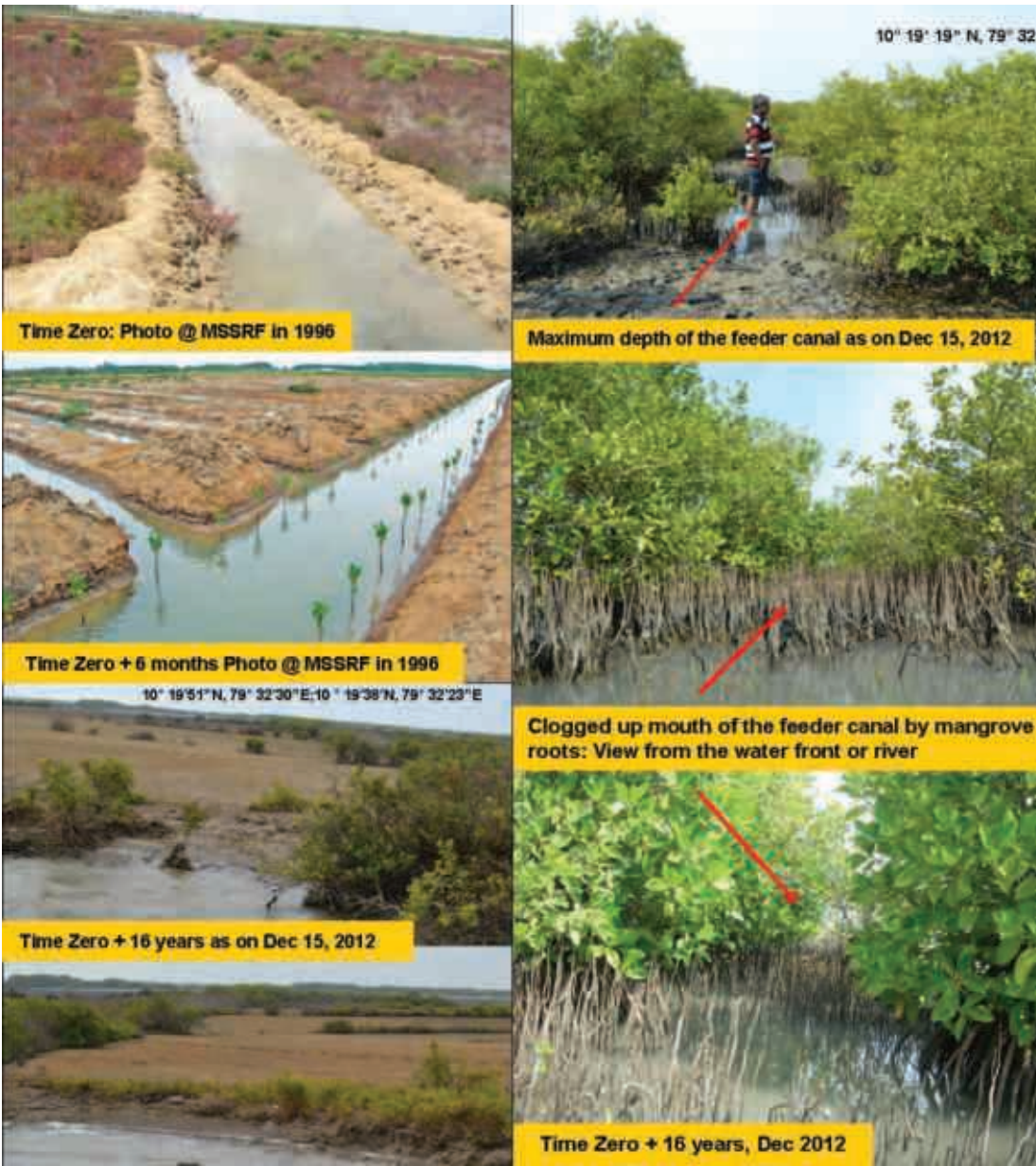
Fig 10.8 Snapshots of developments over time of fishbone canals (This page and next) Initially, canals supported adequate mangrove growth at appropriate substrate elevations. Over time, however, siltation of tidal channels caused mangrove stunting and mortality.
